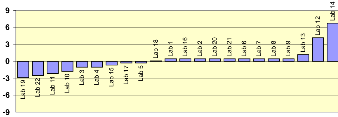
Optimum Moisture Content Between Lab. Z-Score
